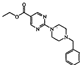
intermediate 1
